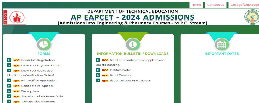
Figure2: Registration Link
